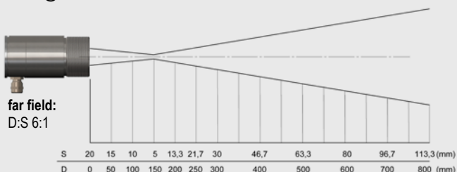
CF2 - optics 30:1 5 mm @ 150 mm
