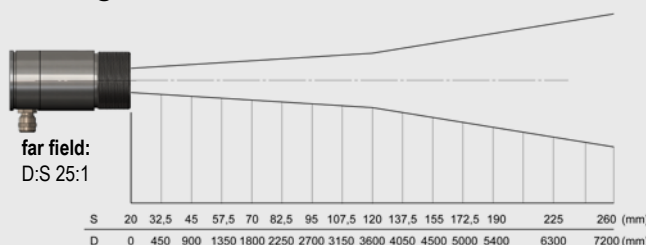
FF - optics 30:1 120 mm @ 3600 mm
