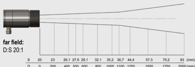
SF - optics 30:1 36.7 mm @ 1100 mm
