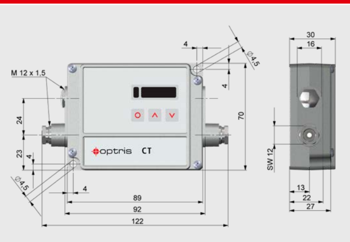
Dimensions electronics
