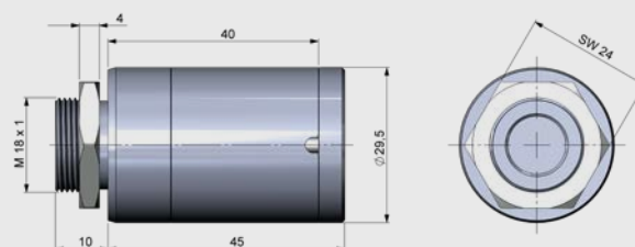
Massive housing
