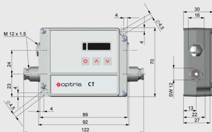
Electronics
