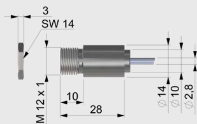
Sensing head
